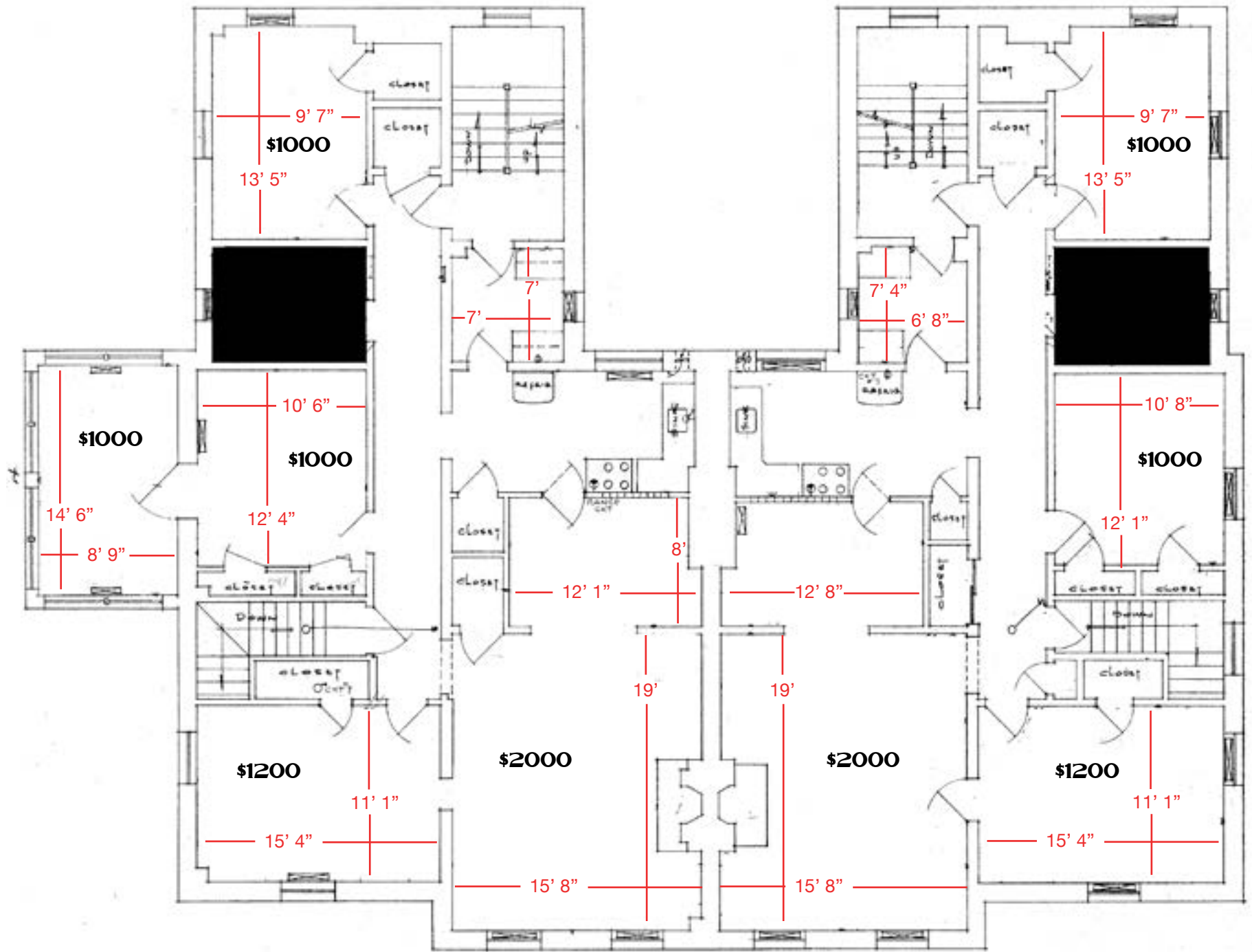
Building 404 - 2nd Floor
